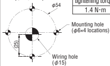
Mounting dimensions (Units:mm)
