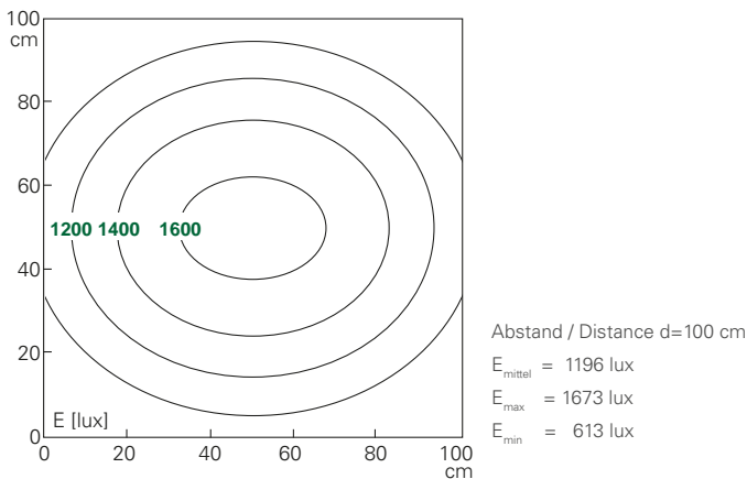
113110-11 / FIELDLED II Einbauversion / integrated version 560mm
