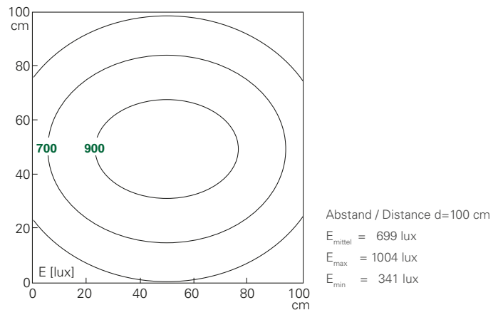
113010-11 / FIELDLED II Einbauversion / integrated version 300mm
